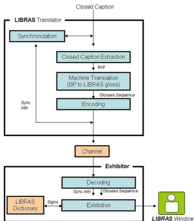
Fig. 1 LibrasTV architecture
