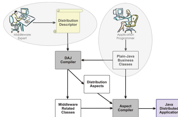
Figure 1. Developing distributed applications using DAJ
