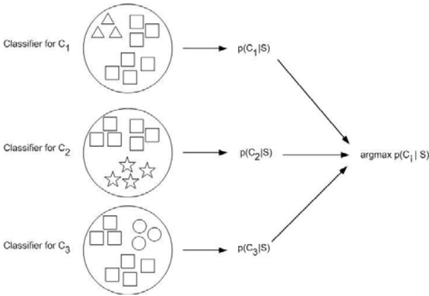
Figure 1. One-Against-All Space Decomposition Approach
