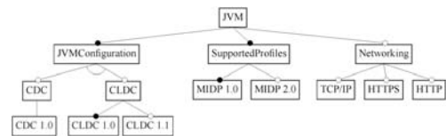
Figure 9: Java Virtual Machine Feature Model
