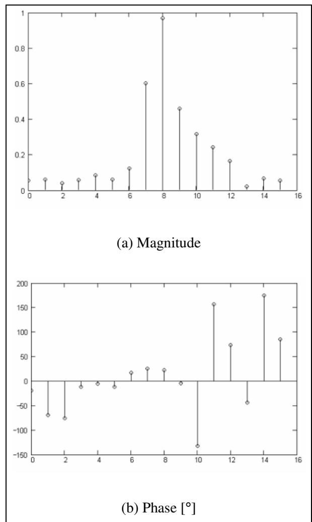
Figure 2: SPIB channel M7 impulse response.
