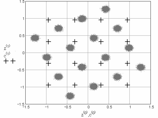
Figure 4: Classical complex valued RBFNN equalizer output y after convergence.
