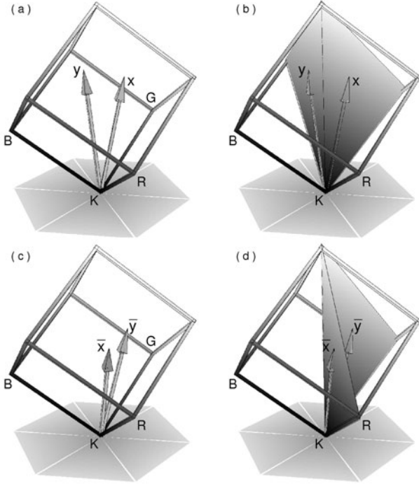
Figure 16. A pair of tones inside the RGB cube. (a) The vector representation for the tones x(t) = 2 \sin[2\pi(468)t] and y(t) = 1.3 \sin[2\pi(585)t + 216(\pi/180)] . (b) The sails for x(t) on the right and for y(t) on the left. (c) The vector representation for the transposed tones \bar{x}(t) and \bar{y}(t) . (d) The sails for \bar{x}(t) and for \bar{y}(t) . (Color online at http://www.cic.unb.br/docentes/arcela/cpv/f16.eps )
