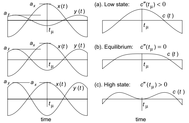
Figure 4. Addition of the spectral components of a m:n -complex in the region of a maximum-minimum coincidence at a time t_\mu . It is shown on the left hand side of the figure the waveforms of a pair of lower and upper components x(t) and y(t) at three different amplitude proportions corresponding respectively (a) to low state, (b) to the equilibrium, and (c) to the high state. On the right hand side, the complex's waveform segments are shown at different states.
