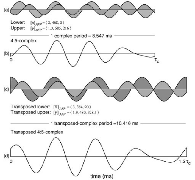
Figure 15. The down transposition of a m : n -complex. (a) Waveforms of the spectral components x(t) = 2 \sin[2\pi(468)t] and y(t) = 1.3 \sin[2\pi(585)t + 216(\pi/180)] . (b) The corresponding 4:5-complex, that is, c(t) = x(t) + y(t) . (c) The transposed components \bar{x}(t) and \bar{y}(t) . (d) The transposed complex has a period 1.22 (the approximate value of q_x ) times greater than that of the untransposed complex and, while it is phase shifted, its waveform has the same shape as the untransposed complex. (Color online at http://www.cic.unb.br/docentes/arcela/cpv/f15.eps )
