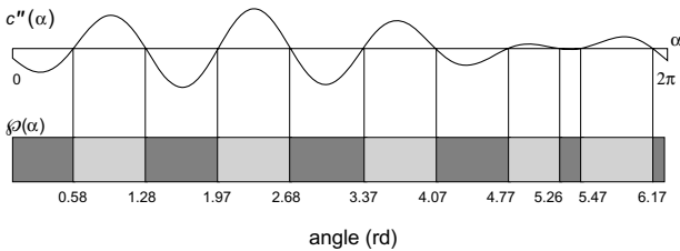
Figure 7. Building of a Boolean zero-crossing pattern from the marks by using dark and light rectangles. A dark rectangle represents a second derivative waveform segment with up concavity, while a light one represents a down concavity segment.
