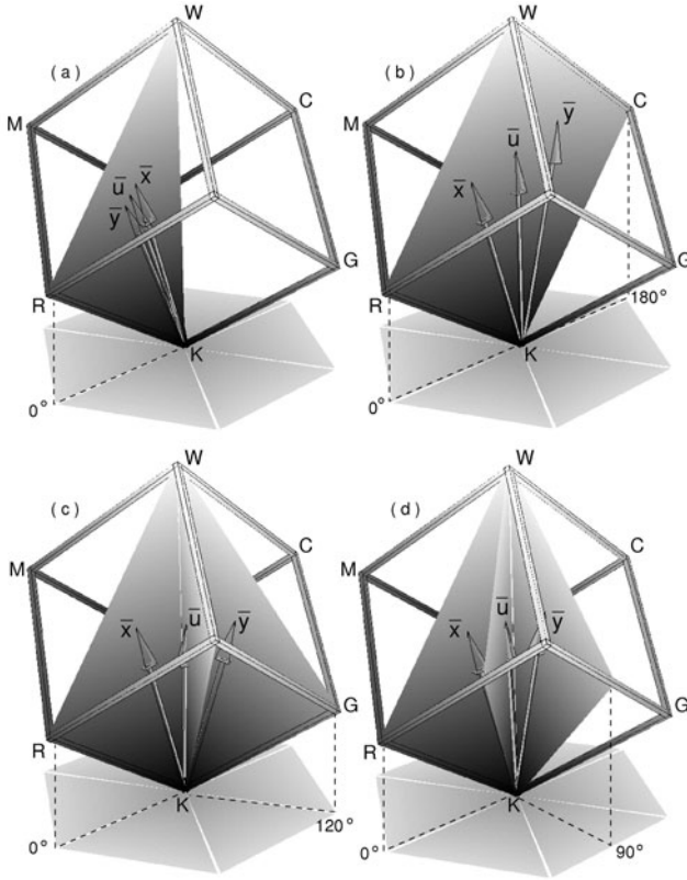
Figure 19. Vector composition of transposed components of m:n -complexes having simple m:n ratio. (a) Vector addition of tones in octaves. (b) Vector addition of tones in fifths. Definition of the red-cyan rectangular section. (c) Vector addition in fourths. (d) Vector addition in major thirds. (Color online at http://www.cic.unb.br/docentes/arcela/cpv/f19.eps )
