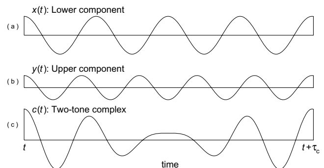
Figure 1. Sinusoid addition of lower and upper components of a two-tone harmonic complex.
