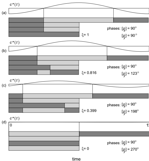
Figure 10. Zero-crossing patterns defined in the second derivative c''(t) of a 1:1-complex having equal-amplitude components for different phase relationships. (a) The full symmetry ( \xi = 1 ) gives the greatest resulting amplitude. This occurs when the phases are such that [p_x] = [p_y] = 90^\circ . (b) With phases [p_x] = 90^\circ , [p_y] = 123^\circ , the resulting amplitude is smaller as a consequence of a smaller symmetry ( \xi = 0.816 ). (c) With phases [p_x] = 90^\circ , [p_y] = 198^\circ , the resulting amplitude is still smaller, due to a still smaller symmetry ( \xi = 0.399 ). (d) A null symmetry ( \xi = 0 ) gives a null resulting amplitude.
