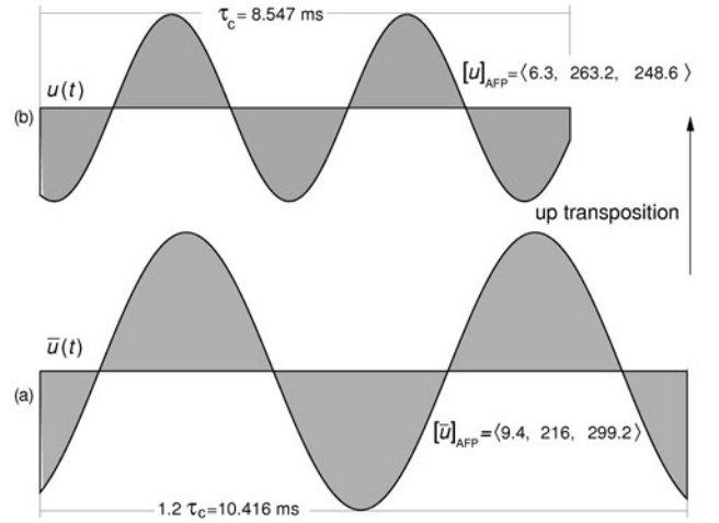
Figure 17. Up transposition. (a) The transposed vector addition tone \bar{u}(t) of components x(t) = 2 \sin[2\pi(468)t] and y(t) = 1.3 \sin[2\pi(585)t + 216(\pi/180)] . (b) The up transposition operation gives the final vector addition tone u(t) , where the frequency is multiplied by the quotient q_x of the original lower tone so that the resulting tone has a period in the same scale of time as that of the original complex. (Color online at http://www.cic.unb.br/docentes/arcela/cpv/f17.eps )
