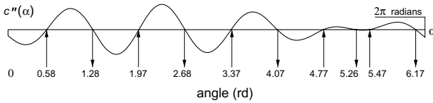
Figure 6. Placement of marks in the zero-crossing angles so as to be oriented according to the curve inclination at these positions.
