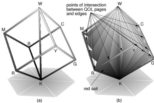
Figure 14. (a) RGB cube with its achromatic diagonal (defined by the vertices K and W, which correspond respectively to the colors black and white) aligned with the vertical direction. Indication of the vertices R, G, B, C, M, and Y which correspond respectively to the colors red, green, blue, cyan, magenta, and yellow. (b) Illustration of some sails as the result of the transformation of some QOL pages into RGB. The red sail contains the vertex R. (Color online at http://www.cic.unb.br/docentes/arcela/cpv/f14.eps )
