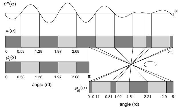
Figure 8. Sectioning of the Boolean zero-crossing pattern \wp(\alpha) into two halves. In order to be compared with the left-half pattern, the right-half one is inverted by a 180^\circ rotation around a vertical axis passing at 3\pi/2 rd so that its mirror image is obtained.
