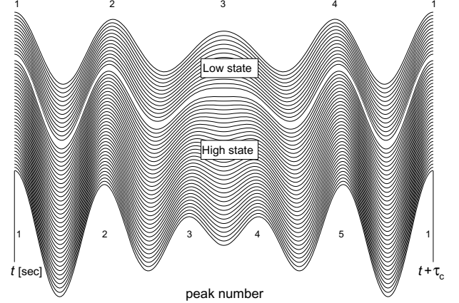
Figure 2. The two possible states in a full period \tau_c of a 4:5-complex along with the equilibrium waveform (the white line) which is the boundary between the regions of low and high states.
