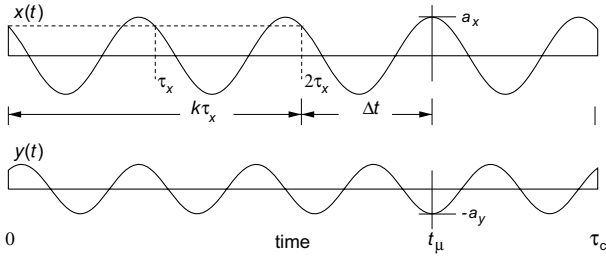
Figure 3. The lower and upper components x(t) and y(t) can be displaced with respect to one another, so that a maximum of one of the sinusoids occurs at the same instant a minimum of the other also occurs. More precisely, to every phase p_x of the lower tone, there is a phase p_y of the upper tone where at a given instant t_\mu a positive peak of x(t) coincides with a negative peak of y(t) . Such maximum-minimum coincidence inside one complex's period \tau_c is shown as occurring at the (k+1) -th period \tau_x of the lower tone.
