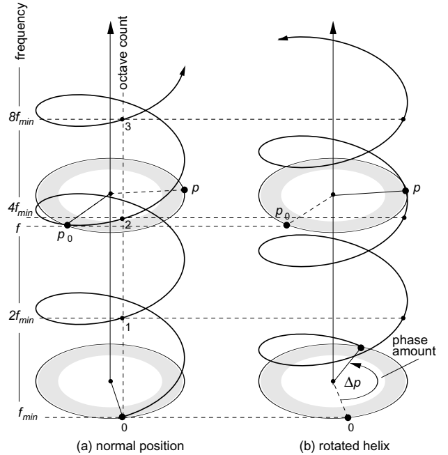
Figure 12. A geometric interpretation of distance in octaves by means of the helix of pitch. (a) The whole number of turns separating the lower limit of pitch f_{min} from the frequency f of the tone. (b) The inclusion of phase in the helix of pitch is such that its effect is to rotate the whole helix by an angle corresponding to its magnitude.
