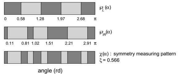
Figure 9. Calculation of the symmetry \xi of the pattern \wp(\alpha) from the average value of the symmetry-measuring pattern \chi(\alpha) which is found after the Boolean exclusive-or operation between of the two half-patterns \wp_L(\alpha) and \wp_{IR}(\alpha) is taken.
