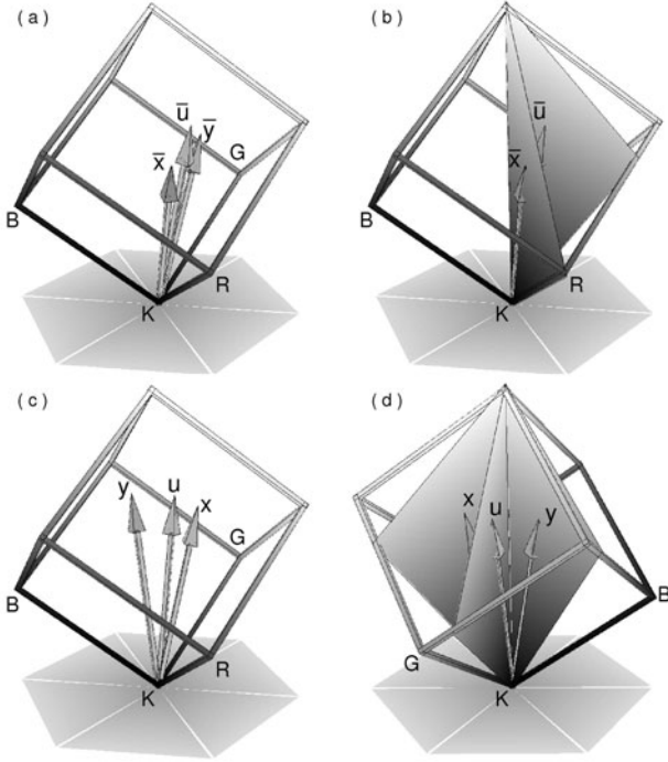
Figure 18. Vector composition of tones. (a) The vector representations [\bar{x}]_{RGB} , [\bar{y}]_{RGB} , and [\bar{u}]_{RGB} of the components x(t) and y(t) along with and transposed vector addition tone \bar{u}(t) . (b) The sails of [\bar{x}]_{RGB} , [\bar{u}]_{RGB} , and [\bar{y}]_{RGB} (the latter is not visible in the figure). (c) The vector representation [\bar{u}]_{RGB} of the vector addition tone u(t) of the components x(t) = 2 \sin[2\pi(468)t] and y(t) = 1.3 \sin[2\pi(585)t + 216(\pi/180)] . (d) The sails for [x]_{RGB} , [y]_{RGB} , and for the addition vector [u]_{RGB} . Here, a 180^\circ rotation has been applied to the cube so as to make all the three sails visible. (Color online at http://www.cic.unb.br/docentes/arcela/cpv/f18.eps )
