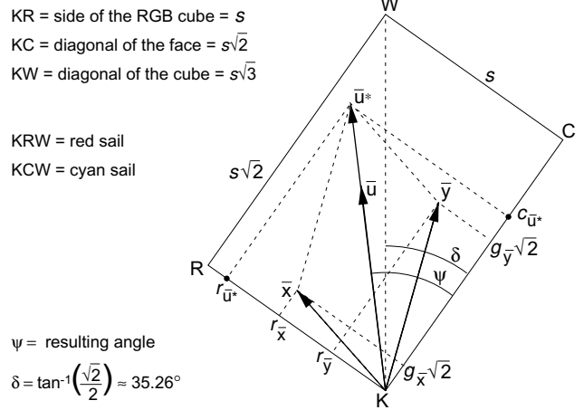
Figure 20. A vector composition on the red-cyan rectangular section of the RGB cube where the resulting transposed vector \bar{u} is found on the red sail. In this case, the vector addition tone will have the same quotient as that of \bar{x} .
