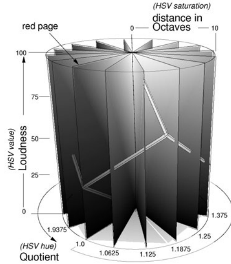
Figure 13. RGB-cube positioning, scaling, and orienting inside the QOL cylinder in a way that its achromatic diagonal coincides with the vertical axis of the cylinder. The vertex R of the cube is positioned on the surface of the cylinder in the same plane as the cylinder [0^\circ] -page (the red-page, i.e., where q = 1 ). In this way, the vertex G is positioned on the [120^\circ] -page, where q = 4/3 ; and the vertex B is positioned on the [240^\circ] -page, where q = 5/3 . Although the cylinder is shown with a finite number of pages, the angular spacing is continuous, so that to any quotient between 1 and 2 there is a corresponding page. (Color online at http://www.cic.unb.br/docentes/arcela/cpv/f13.eps )
