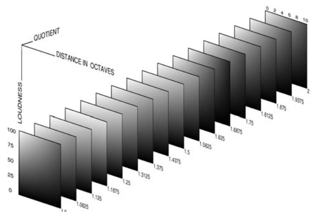
Figure 11. Rectangular QOL organization of tones into pages, each of them corresponding to a different quotient in the range 1 \leq q < 2 . Each page is a Cartesian coordinate system of distance in octaves versus loudness, that is, a rectangle where all tones having the same quotient are located. (Color online at http://www.cic.unb.br/docentes/arcela/cpv/f11.eps )
